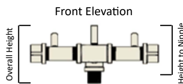
(Front Elevation Dimensions: Overall 3 5/8" H, 2 3/8" nipple)
